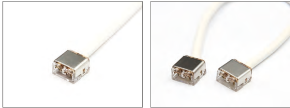
IP20 connector 10A(tape to wire) 110501010212 IP20 Jumper connector 10A (tape-wire-tape) 110501010213
