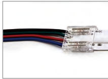
Connector with cables 110501010580
