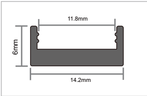
PC Channel 160103010066
